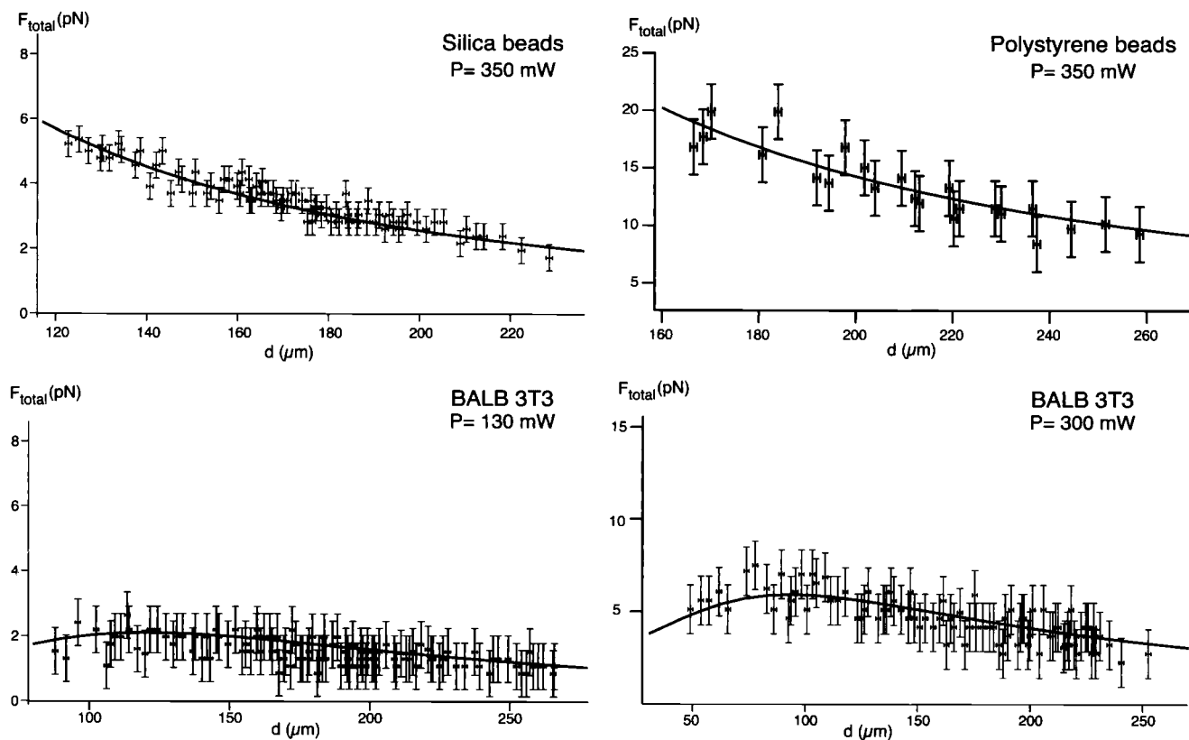
FIGURE 8 The total forces from one laser beam on silica beads, polystyrene beads, and BALB 3T3 fibroblasts as functions of the distance d between the fiber tip and the object. The data points are from measuring the total force on the objects in the optical stretcher after obstructing one of the laser beams. The solid lines represent the total forces calculated using ray optics. The radii of the silica beads, the polystyrene beads, and the fibroblasts were \rho = 2.50 \pm 0.04 \mu\text{m} , \rho = 2.55 \pm 0.04 \mu\text{m} , and \rho = 7.70 \pm 0.05 \mu\text{m} , and the refractive indices were n_2 = 1.430 \pm 0.003 , n_2 = 1.610 \pm 0.005 , and n_2 = 1.370 \pm 0.005 , respectively. The total light power P is indicated in each case. The error bars represent standard deviations; the error in the distance measurement was \pm 0.6 \mu\text{m} .
