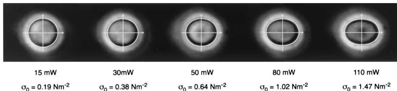
FIGURE 11 Comparison between the deformations of RBCs observed in the optical stretcher and the deformations expected from membrane theory (white lines). The peak stresses \sigma_0 calculated using ray optics, which are shown with each image, were used for the membrane theory calculations. The resulting theoretical shapes, calculated with Eq. 13a, were overlaid on the original images from Fig. 9 to show the excellent agreement between the two for all peak stresses.
