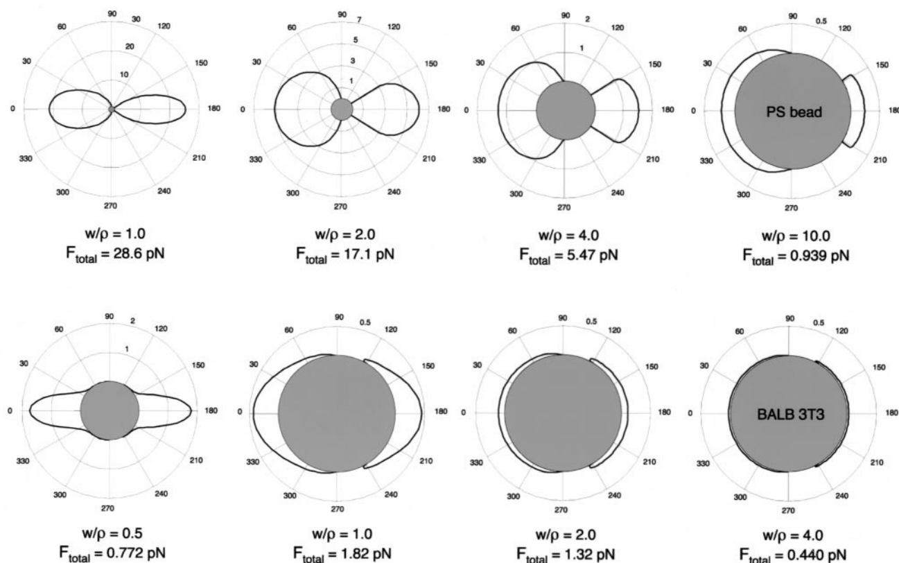
FIGURE 6 Surface stress profiles for one laser beam incident from the left on a polystyrene bead ( top row ) and a BALB 3T3 fibroblast ( bottom row ) for different ratios between the beam radius w and the object's radius \rho . The radii of the polystyrene bead and the fibroblast used for this calculation were \rho = 2.55 \mu\text{m} and \rho = 7.70 \mu\text{m} and the refractive indices were n_2 = 1.610 and n_2 = 1.370 , respectively. The total light power P = 100 \text{ mW} for all profiles. The concentric rings indicate the stress in \text{Nm}^{-2} (note the different scales). The resulting total force after integration over the surface acting on the center of gravity of the object is noted in each case.
